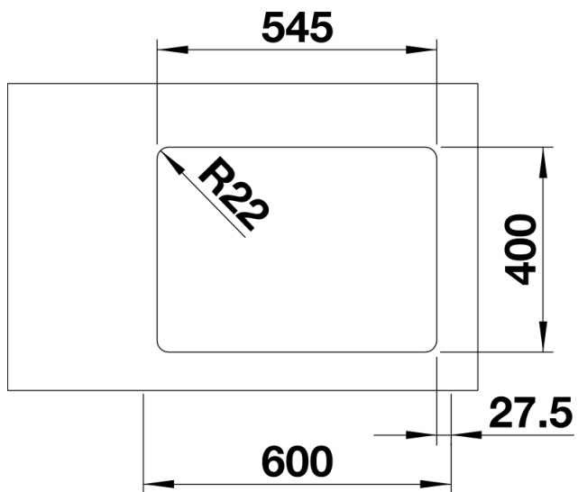
Cut-out
