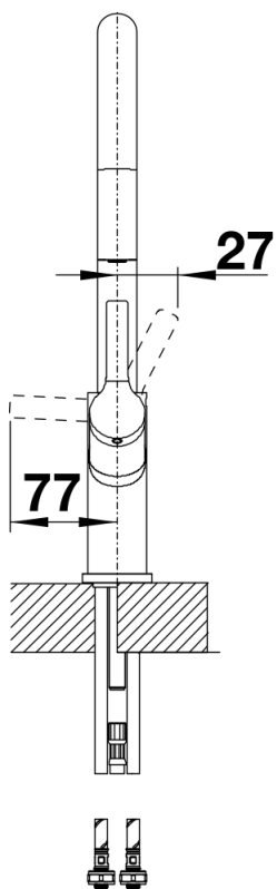
Side view hand gear 2D
